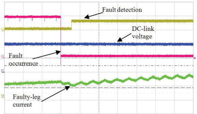
Fig. 24. Fault detection in case 1- from top to bottom: fault- fault detection- DC voltage (100V/div)- faulty phase current (5A/div)-time scale:200 \mu\text{s} /div.
