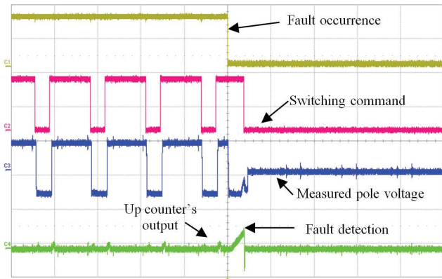
Fig. 27. Fault detection signals in case 1- from top to bottom: fault occurrence- switching command T_1 - measured pole voltage V_{a1o,m} (200V/div)- up-counter's output in the detection block. Time scale: 100 \mu s/div.
