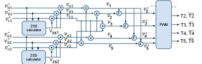
Fig. 6. Principle of PWM and new reference voltage generation for the four healthy legs after a fault in the leg 1.
