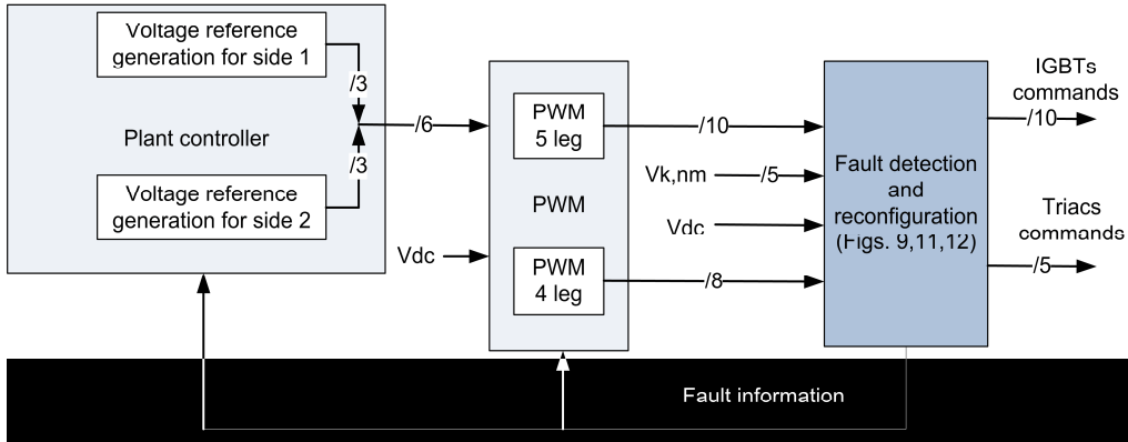
Fig. 10. Proposed reconfigurable control.
