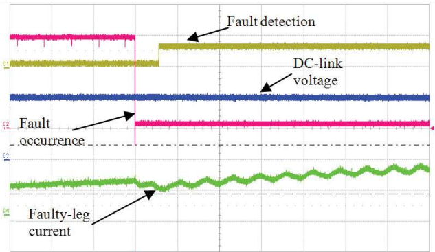
Fig. 24. Fault detection in case 1- from top to bottom: fault- fault detection- DC voltage (100V/div)- faulty phase current (5A/div)-time scale:200 \mu\text{s}/\text{div} .
