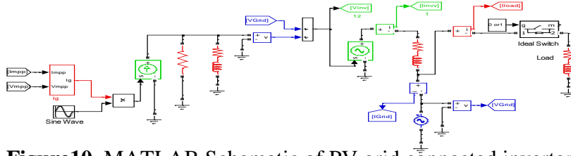
Figure10. MATLAB Schematic of PV grid connected inverter.
