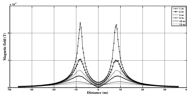
Figure 6. Magnetic field for horizontal configuration with varying height
