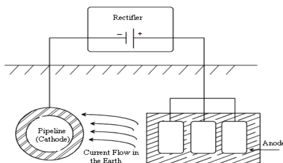
Figure 15. Impressed current cathodic protection System
