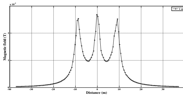
Figure 4. Magnetic field for horizontal configuration
