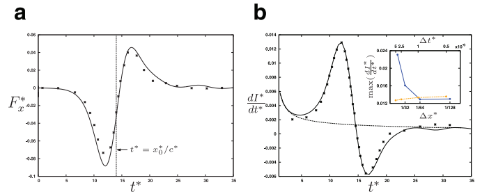
Fig. 6. Solitary wave propagating over a semi-circular cylinder: Evolution of (a) the drag force F_x^* exerted by the fluid on the cylinder, and (b) the time derivative of the spatially-averaged horizontal momentum: (—), present study; (---), results of [3]; (· · · · ·), present results for the case of a solitary wave propagating over a flat bottom. The variation of the maximum value of dI^*/dt^* as a function of the time step (· · · · ·) and the grid size (—) in the region of the cylinder is included in (b) to show the convergence of the computation. Here, I^* = I/cM .
