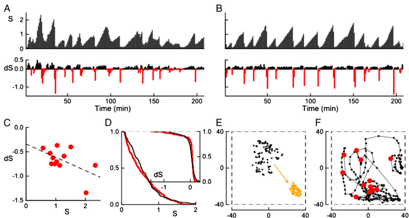
Fig. 1. (A) Experimental time series of the group area S(t) ( \times 1,000 m 2 ) and its changes over 1 min dS(t) ( \times 1,000 m 2 ) as a function of time. S(t) displays the intriguing ratchet-like temporal patterns with slow increases, corresponding to dS(t) \geq 0 (in black), abruptly interrupted by fast packing events corresponding to dS(t) \ll 0 (in red). (B) Same quantities as obtained from a typical simulation of our model (see Numerical Simulations ). (C) Parametric plot of dS(t) vs. S(t) for the major packing events ( dS(t) \leq -0.35 \times 1,000 m 2 ). The dashed line marks linear regression with a linear coefficient equal to -0.27 (with a P value of 0.07). (D) Empirical CCDF of S(t) (black), compared with the model one extracted from B (red). (Inset) CCDFs of experimental dS(t) (black) and model prediction (red). (E) Two typical experimental snapshots are shown within paddock boundaries (fence, dotted line): a dispersed group (at t = 110 min, black dots) immediately precedes a packing event, and a compact one (at t = 112 min, orange dots) follows it. (F) Trajectory of the center of mass of the experimental group. The red dots mark the starting position of the major packing events. The observation tower is located outside the fence, near the bottom left corner of E and F. Error bars for S , dS , and the center of mass positions due to individual sheep tracking errors are negligible on the shown scales.
