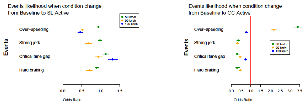
Figure 4: Odds ratio for automatically detected safety critical events when condition change from baseline to SL (a) or CC active (b).
