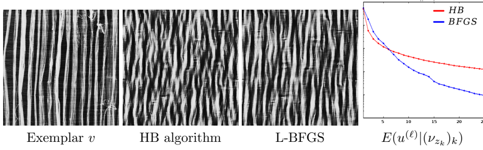
Fig. 3.2: Synthesis results u^{(\ell)} obtained after \ell = 25 iterations of HB algorithm and L-BFGS.
