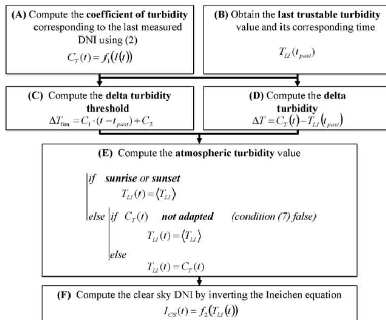
Fig. 2. Diagram of the developed knowledge model.
