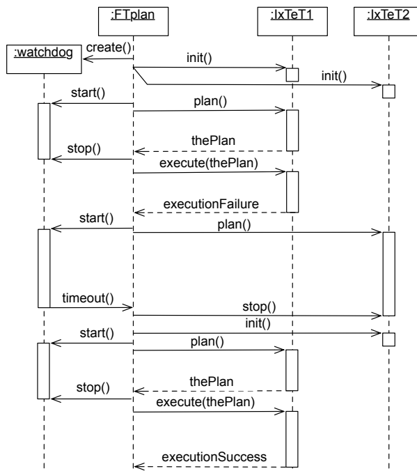
Figure 4. A fault tolerance scenario
