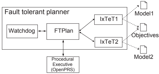
Figure 3. Fault tolerant planner
