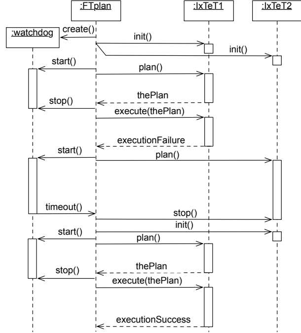
Figure 4. A fault tolerance scenario
