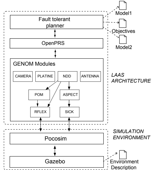
Figure 5. Simulation environment
