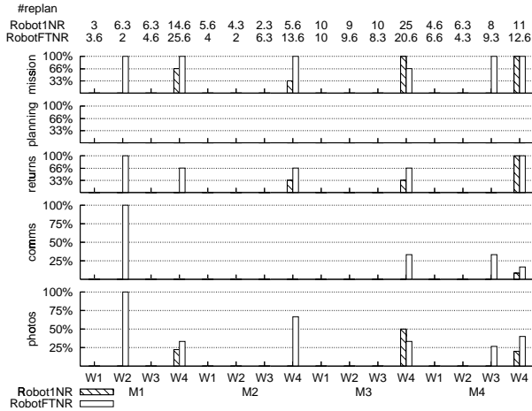
Figure 7. Effect of additional replanning
