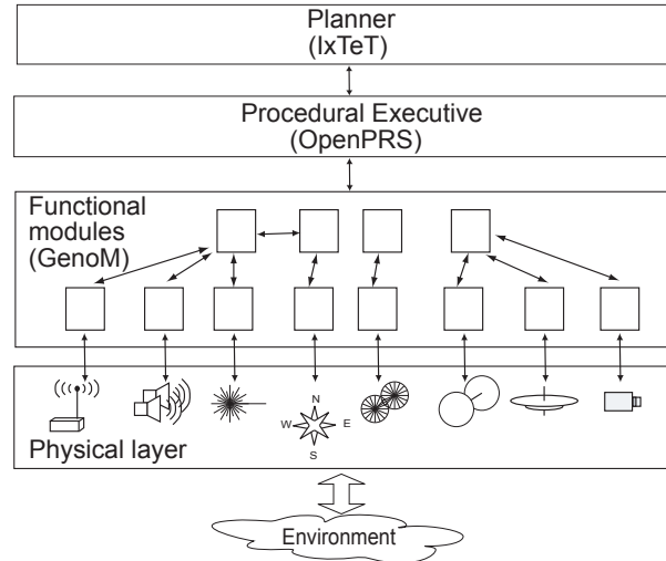
Figure 2. The LAAS architecture
