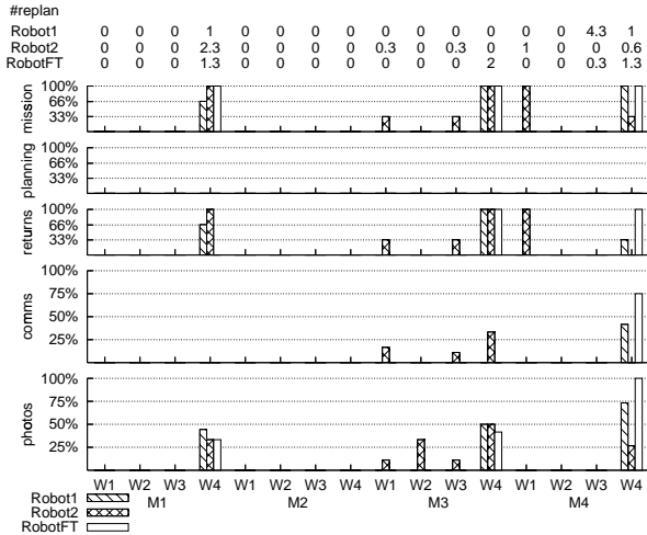
Figure 6. Impact of FTplan on performance
