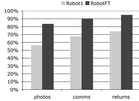
Figure 8. Goal success levels (29 mutations)
