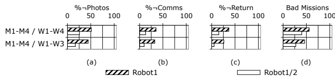
Figure 7: Impact of planner redundancy (with injected faults)
