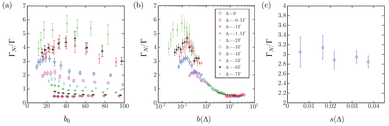
FIG. 3. (color online). Experimental study of the initial collective decay rate \Gamma_N . (a) Systematic analysis of \Gamma_N as a function of the resonant optical thickness b_0 and the detuning \Delta . (b) Same data shown as a function of b(\Delta) . When b(\Delta) \gtrsim 1 , it becomes the scaling parameter. (c) \Gamma_N as a function of the saturation parameter s(\Delta) , for b_0 = 21 \pm 1 and \Delta = -4\Gamma . In all panels, errorbars represents the 95% confidence interval of the fit.
