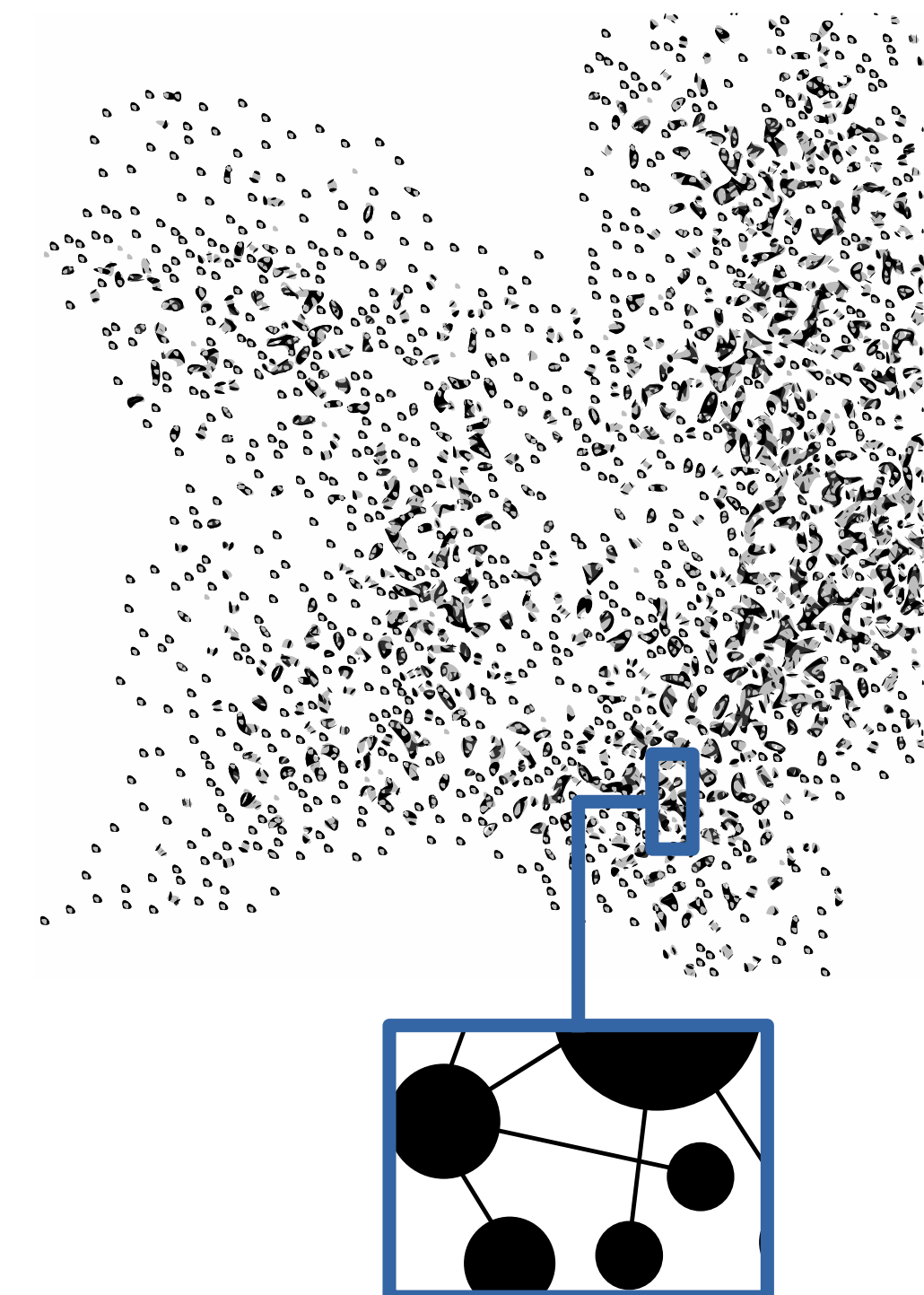
A partly connected network
