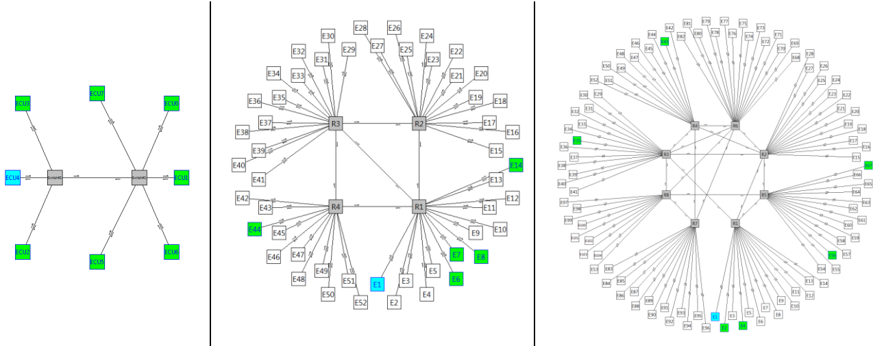
Figure 1: topology of case-study #1 (Daimler prototype network), case-study #2 (medium AFDX network) and case-study #3 (large AFDX network). A multi-cast stream is shown on each topology.
