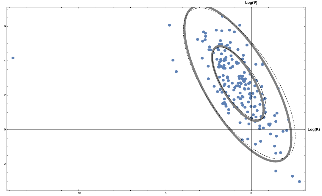
FIGURE 7.2. In black: 50% and 95% confidence ellipsoids for the reference distribution \mathcal{N}(\mu_B, \Sigma_B) ; in gray: same confidence ellipsoids for the distribution \mathcal{N}(\widehat{\mu}_B, \widehat{\Sigma}_B) obtained from the mixture distribution \mathcal{M} . Dots correspond to the parameters of the “NB species”, estimated by PHD_h . PHD h : theoretical versus empirical distribution of (K,p)
