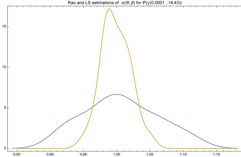
FIGURE 7.6. The Willams-Rao's condition in the aggregative case - the blue density is \frac{\alpha_{Rao}}{K\beta} ; the yellow one is \frac{\alpha_{LS}}{K\beta}
