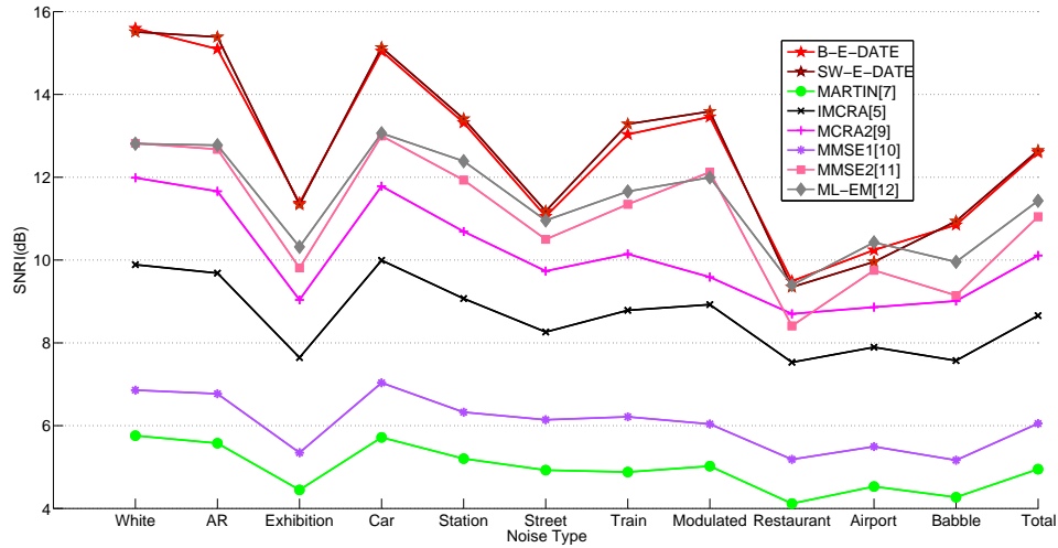
Fig. 6: SNRI with various noise types
