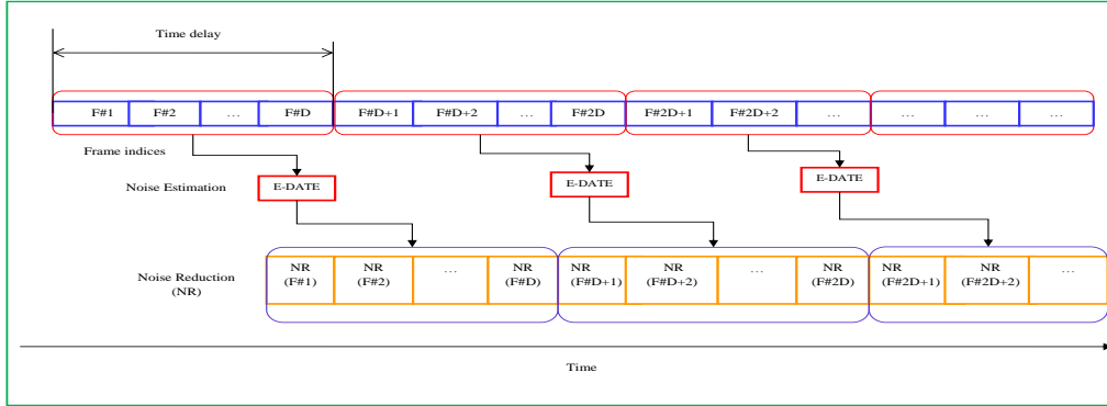
Fig. 3: Block E-DATE (B-E-DATE) combined with noise reduction (NR). A single noise power spectrum estimate is calculated every D non-overlapping frames and used to denoise each of these D frames.
