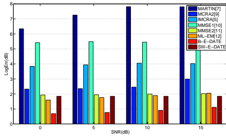
(a) white gaussian noise
