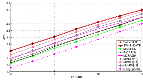
(a) white gaussian noise
