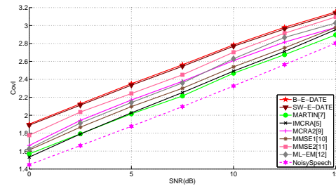
(b) AR noise
