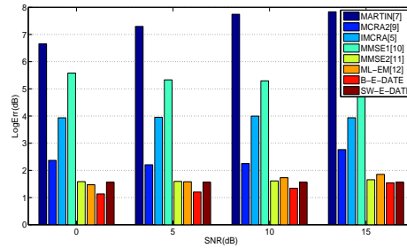
(b) AR noise
