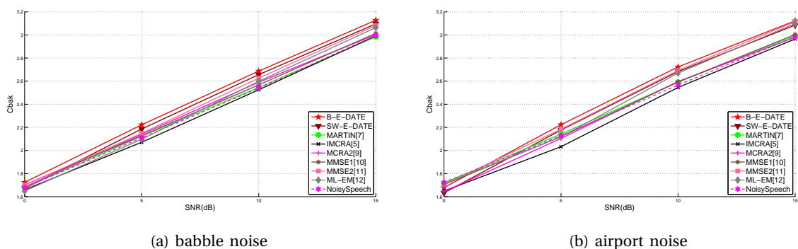
Fig. 8: Speech quality evaluation after speech denoising ( C_{bak} composite criterion).
