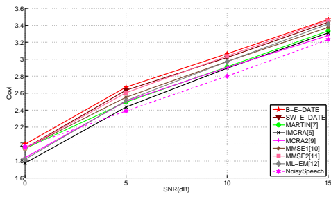
(e) station noise
