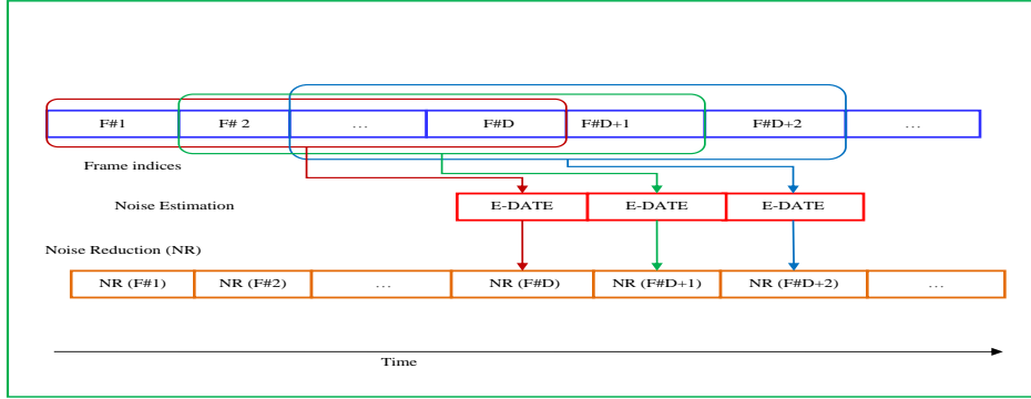
Fig. 4: Sliding-Window E-DATE (SW-E-DATE) combined with noise reduction. For the first D-1 frames, a surrogate method for noise power spectrum estimation is used in combination with noise reduction. Once D frames are available and upon reception of frame D+\ell , \ell \geq 0 , the SW-E-DATE algorithm provides the NR system with a new estimate of the noise power spectrum computed using the last D frames F_{\ell+1}, \dots, F_{\ell+D} for denoising of the current frame.
