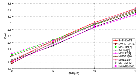
(h) airport noise
