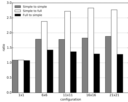
Fig. 13: With-adaptiveness-over-without-adaptiveness ratio.
