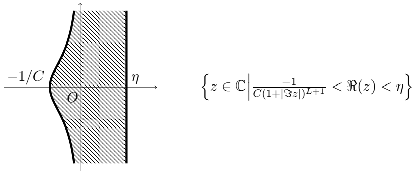
FIGURE 1. Shape of \mathcal{D}_{\eta,C,L}
