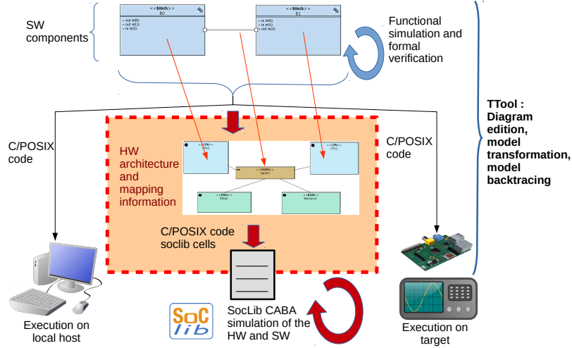
Figure 1. Overview of model transformations for simulation, verification and code generation/execution. Bracktracing to models is not presented, but is effectively implemented in TTTool.
