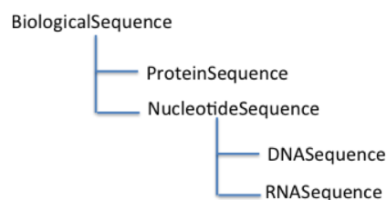
Figure 4: Fragment of the myGrid Ontology.
