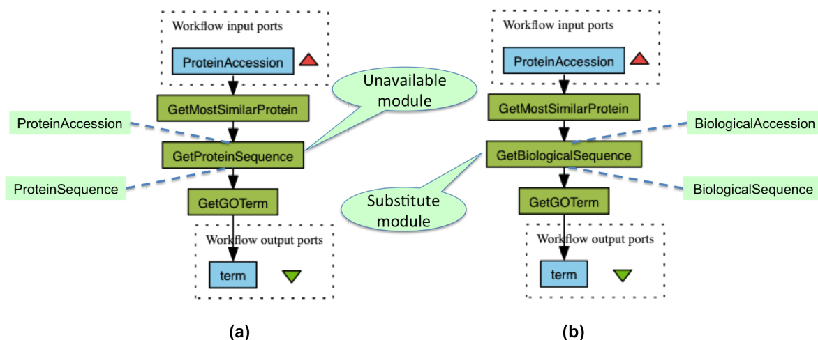
Figure 7: Example of a substitute module that does not have semantically equivalent input and output as the unavailable module.
