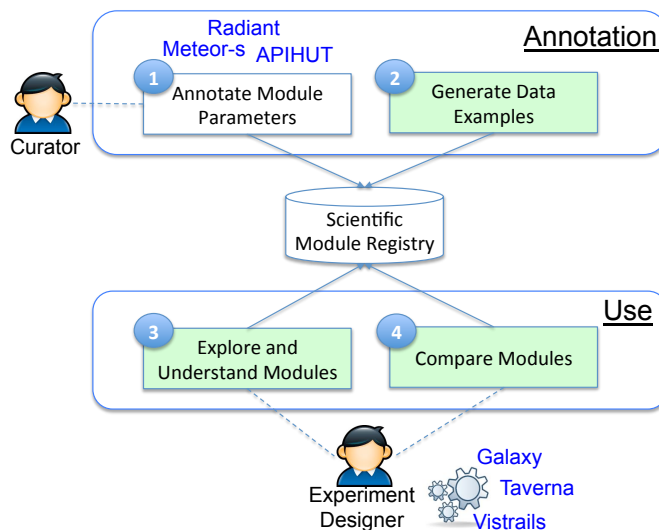
Figure 3: Overall architecture.
