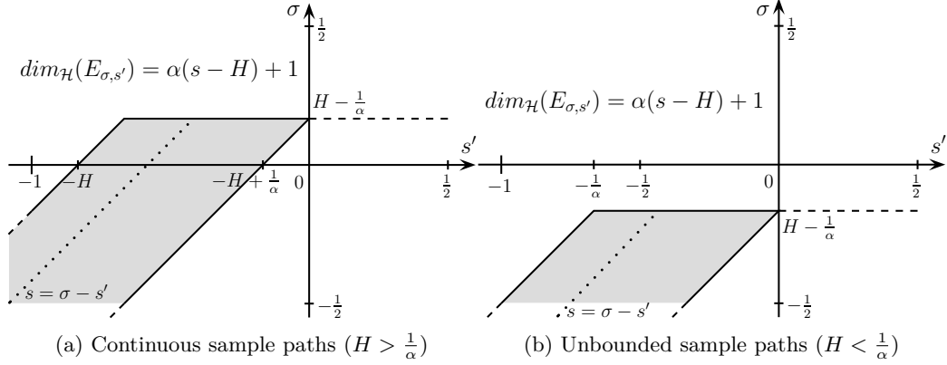
Figure 1: Domains of admissible 2-microlocal frontiers for the LFSM
