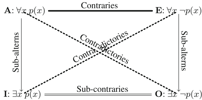
Fig. 1. Square of opposition
