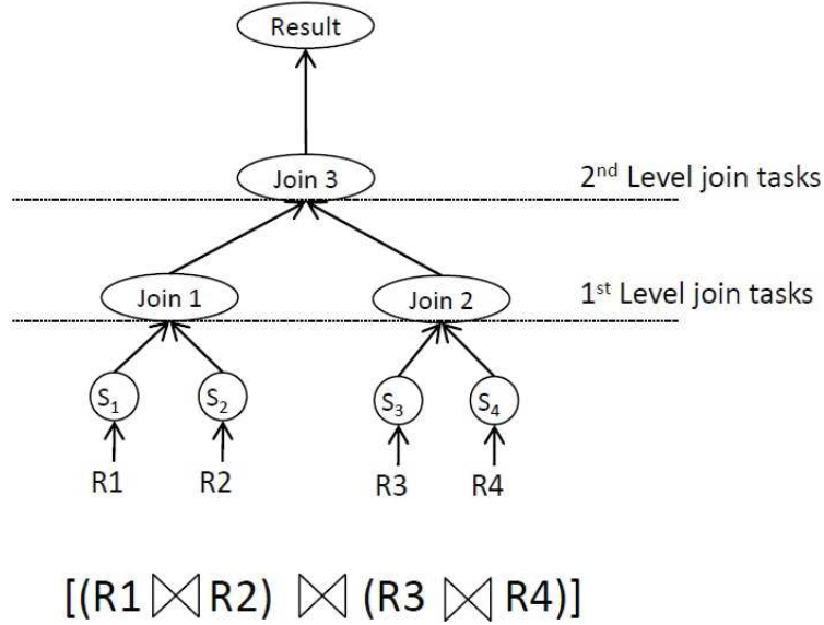
Figure 1 An example query and its query tree
