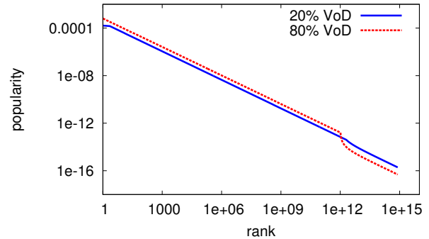
Figure 4: Popularity laws for a composition of 1 TB catalogue, representing VoD, and 1 PB catalogue, representing all other content; both catalogues have Zipf(.8) popularity and the relative traffic volumes are 20:80 and 80:20, respectively.
