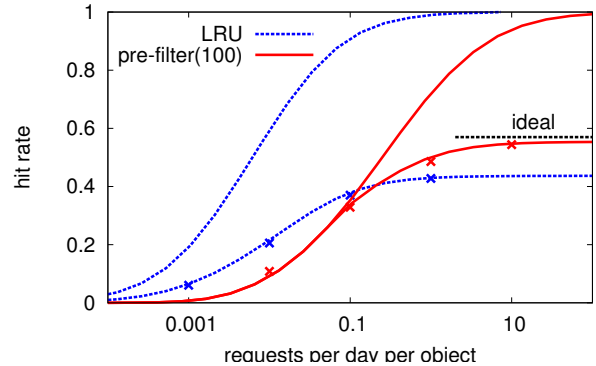
Figure 3: Hit rate against normalized demand \sigma : analytical results for a cache of size 1000 and an unlimited cache for LRU and LRU+pre-filter of 100; simulation results are shown as crosses for C = 1000 ; N = 10^4 items with Zipf(.8) popularity.
