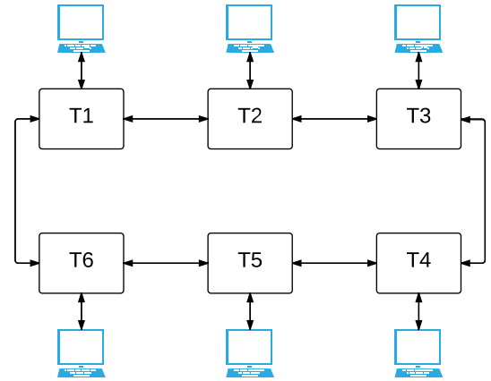
Fig. 1. AeroRing network
