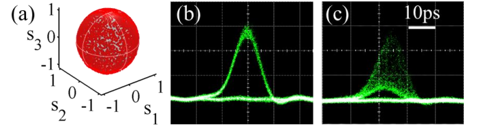
Fig. 8 Poincaré sphere (a) and eye-diagram (b) of the 10-Gbit/s signal recorded at the output of Fiber-1 ( L = 5.3 km; losses 0.24 dB/km; \gamma = 1.7 W ^{-1} km ^{-1} ) for an input average power of 15 dBm and a backward power of 30 dBm. Panel (c): output eye-diagram for a backward power of 35 dBm.
