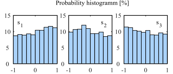
Fig. 7 :Experimental probability histogram (%) of the 3 normalized Stokes parameters s_1 , s_2 and s_3 . The input power is P_S(0) = 15 dBm; the backward power is P_J(L) = 33 dBm; the fiber under test is Fiber-1 ( L = 5.3 km; losses 0.24 dB/km; \gamma = 1.7 W ^{-1} km ^{-1} ). The corresponding Poincaré sphere is represented in Fig. 6(d).
