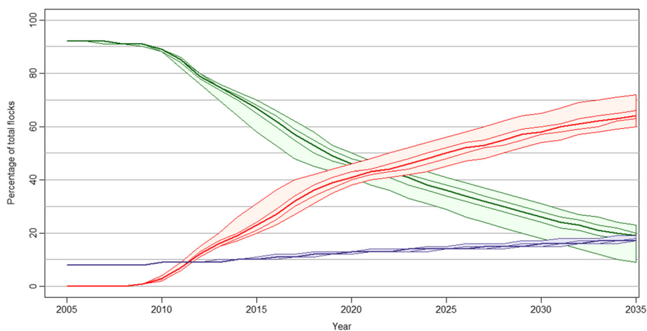
Figure 2 Simulated development of severe footrot in Norwegian sheep flocks without an elimination programme. The percentage of susceptible (green), infected (red) and low susceptible (purple) flocks are shown for each of the years 2005 – 2035 with the median value and 2.5, 25, 75 and 97.5 percentiles.
