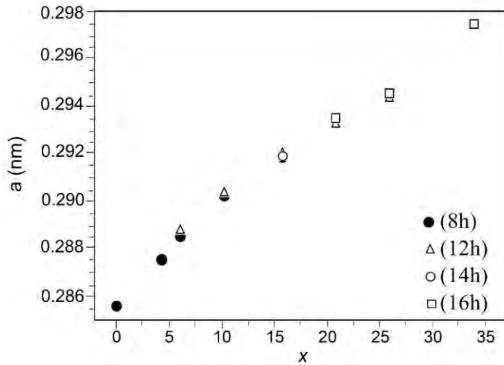
Figure 2 – Evolution with tin content of the lattice parameter of the bcc phase of as-milled Fe_{53.3-0.6x}Co_{46.7-0.4x}Sn_x (milling times range from 8h to 16h).
