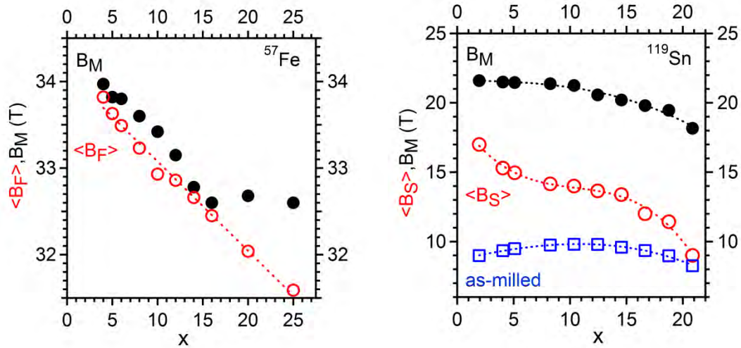
Figure 11 - As-milled (10h) \text{Fe}_{53.3-0.6x}\text{Co}_{46.7-0.4x}\text{Sn}_x annealed at 673K for 15h: ^{57}\text{Fe} (left) and ^{119}\text{Sn} (right) HMF's at RT: \langle B_F \rangle and \langle B_S \rangle (empty circles), and B_M (solid circles) as a function of x . For comparison, \langle B_S \rangle is shown for as-milled alloys (right, empty squares) (the associated B_M almost coincides with it). (color online).
