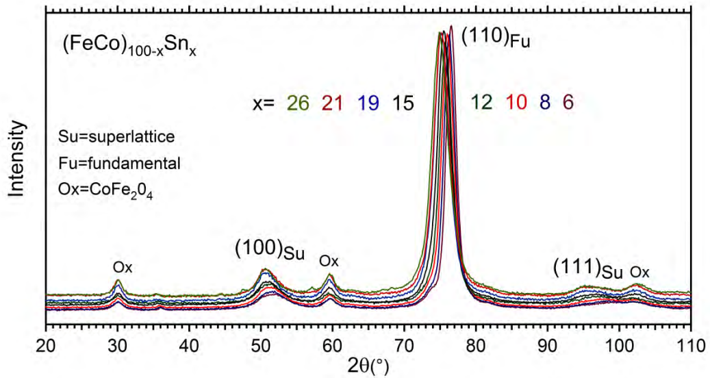
Figure 6 - Neutron diffraction patterns ( \lambda = 0.252 nm) of as-milled \text{Fe}_{53.3-0.6x}\text{Co}_{46.7-0.4x}\text{Sn}_x ( 6 \leq x \leq 26 ) annealed at 673K for 15h. (color online)
