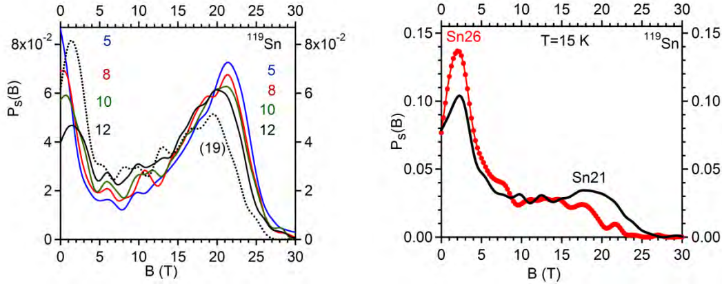
Figure 10 - ^{119}\text{Sn} hyperfine magnetic field distributions of as-milled (10h) \text{Fe}_{53.3-0.6x}\text{Co}_{46.7-0.4x}\text{Sn}_x annealed at 673K for 15h (right) : (left) distributions at RT for the indicated values of x and (right) distributions at 15K for x=21, 26 . (color online).
