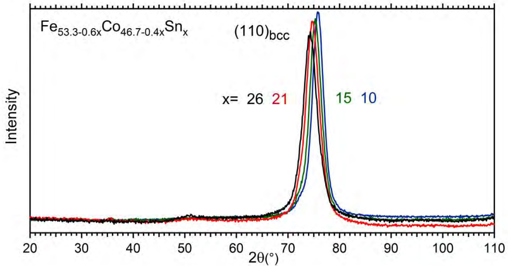
Figure 3 - Neutron diffraction patterns ( \lambda = 0.252 nm) of as-milled (10h) \text{Fe}_{53.3-0.6x}\text{Co}_{46.7-0.4x}\text{Sn}_x for the indicated values of x ( x increases from right to left). (color online)
