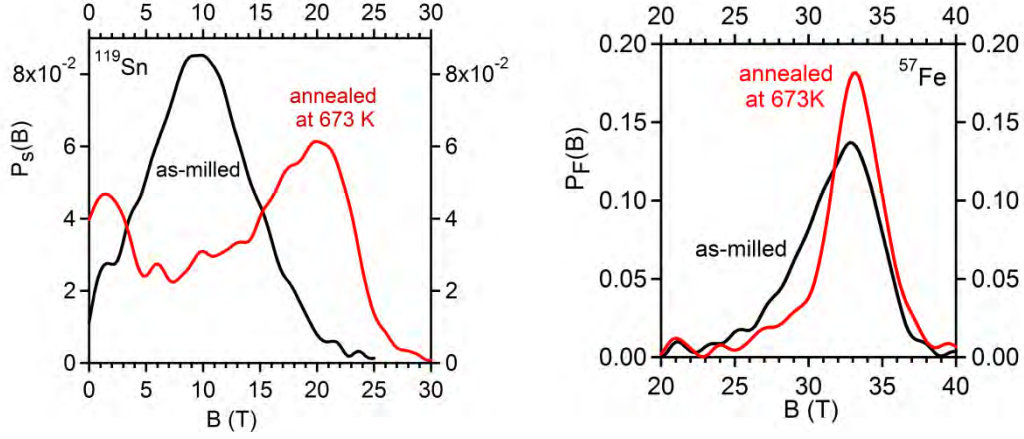
Figure 9 - RT hyperfine magnetic field distributions ( ^{119}\text{Sn} : left, and ^{57}\text{Fe} : right) of \text{Fe}_{46}\text{Co}_{42}\text{Sn}_{12} : in the as-milled state (10h) and after annealing at 673K for 15h. (color online).
