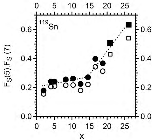
Figure 12 - As-milled (10h) \text{Fe}_{53.3-0.6x}\text{Co}_{46.7-0.4x}\text{Sn}_x annealed at 673K for 15h: Fraction at RT of ^{119}\text{Sn} atoms whose HMF's are either less or equal to 5 T (empty circles) or less or equal to 7 T (solid circles), as a function of x for x \leq 19 . The values at 15K are plotted for x=21, 26 (empty squares for 5 T and solid squares for 7 T). The dashed lines are guides to the eye.
