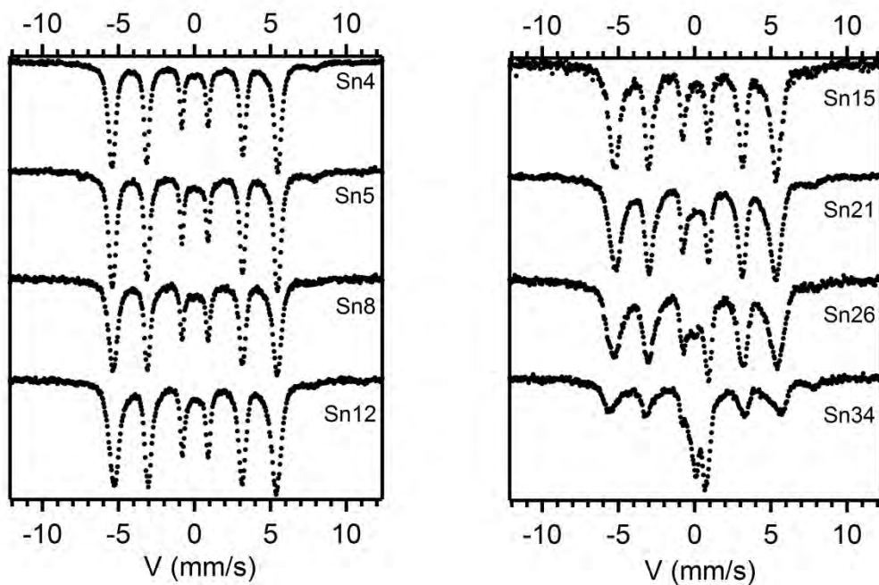
Figure 7 - RT ^{57}\text{Fe} Mössbauer spectra of as-milled (10h) \text{Fe}_{53.3-0.6x}\text{Co}_{46.7-0.4x}\text{Sn}_x annealed at 673K for 15h.
