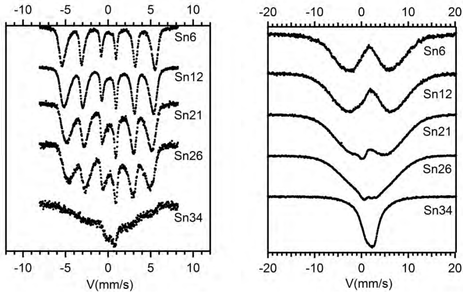
Figure 4 - RT ^{57}\text{Fe} Mössbauer spectra (left) and ^{119}\text{Sn} Mössbauer spectra (right) of as-milled (10h) \text{Fe}_{53.3-0.6x}\text{Co}_{46.7-0.4x}\text{Sn}_x for the indicated values of x .
