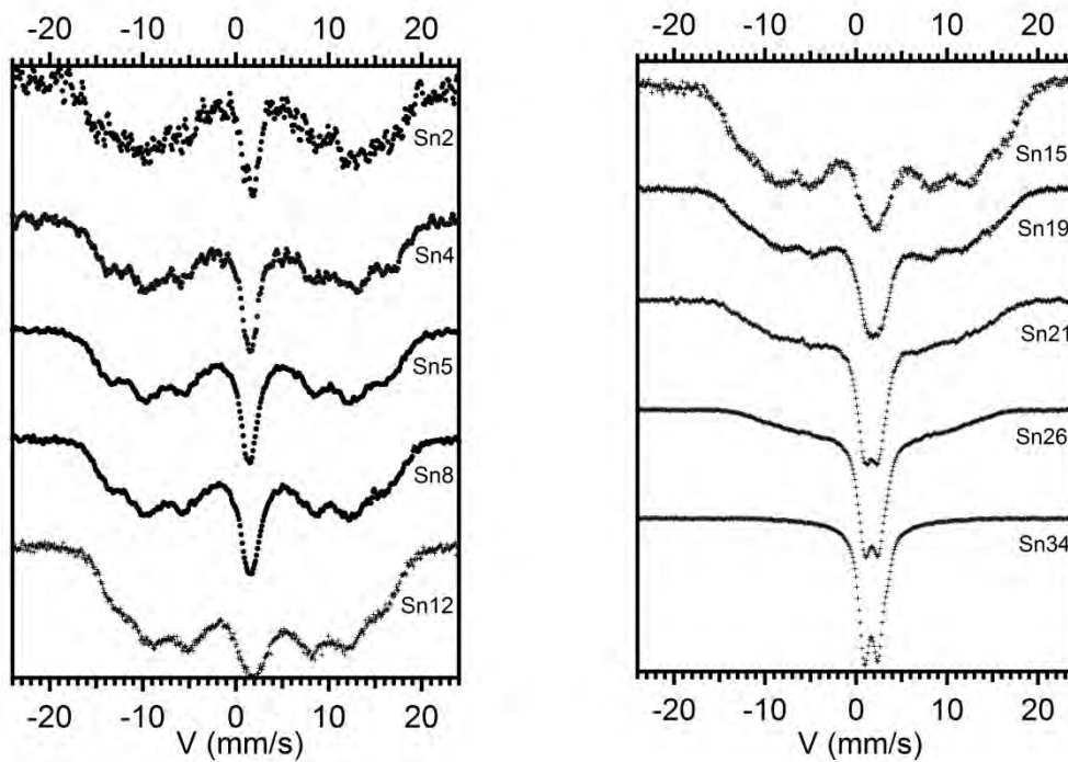
Figure 8 - RT ^{119}\text{Sn} Mössbauer spectra of as-milled (10h) \text{Fe}_{53.3-0.6x}\text{Co}_{46.7-0.4x}\text{Sn}_x annealed at 673K for 15h.
