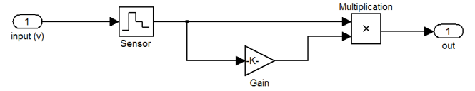
Figure 3: Blocks introducing a uniform noise in a sensor.
