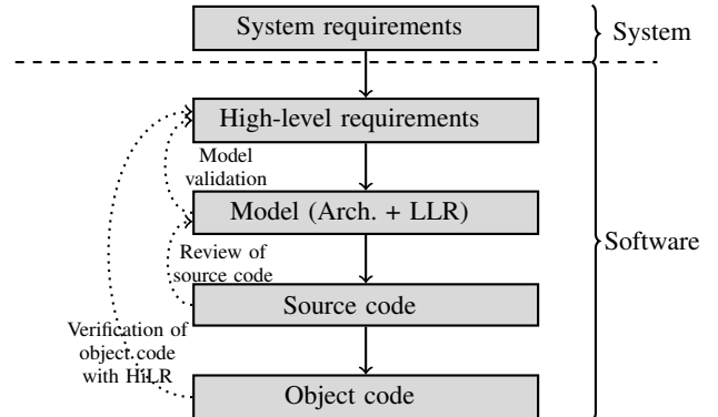
Figure 1: Simplified life-cycle in model-based development.
