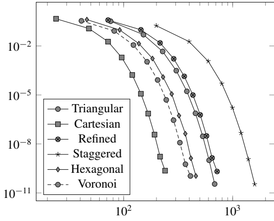
(a) \|u_h - \hat{u}_h\|_{a,h} vs. N_{\text{dof}}
