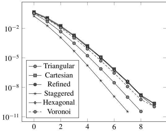
(c) \|u_h - \hat{u}_h\|_{a,h} vs. p
