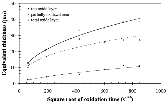
Fig. 10. Oxidation kinetics of the Si 3 N 4 -TiN ceramic under thermal aging tests in air at 1150 °C.
