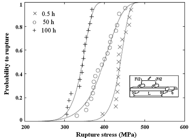
Fig. 12. Results of the room temperature 4-points bending tests performed on Si 3 N 4 -TiN specimens pre-oxidized at 1150 °C during 0.5 h, 50 h and 100 h: graphic representation of the probability of failure as a function of the rupture stress.
