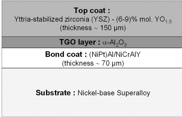
Fig. 13. Laminate structure and composition of the thermal barrier coatings elaborated by EB-PVD process.
