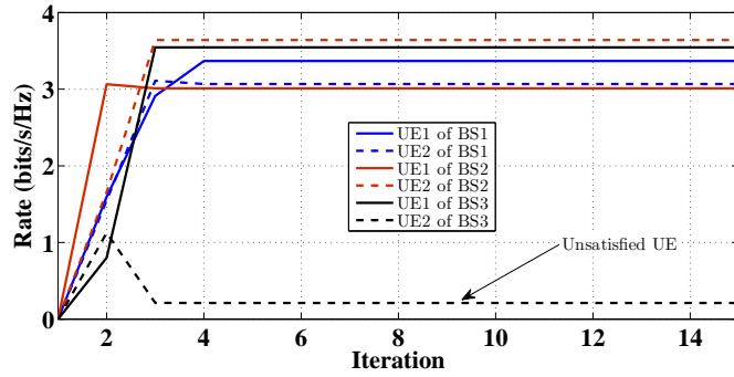
(b) A 5-GSE in pure strategies for \tau_i = [3]\text{bits/s/Hz} and \bar{\tau}_i = [5]\text{bits/s/Hz} .
