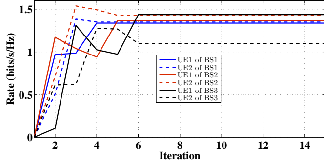
(a) Pure strategy SE for \tau_i = 1\text{bits/s/Hz} and \bar{\tau}_i = 3\text{bits/s/Hz} .
