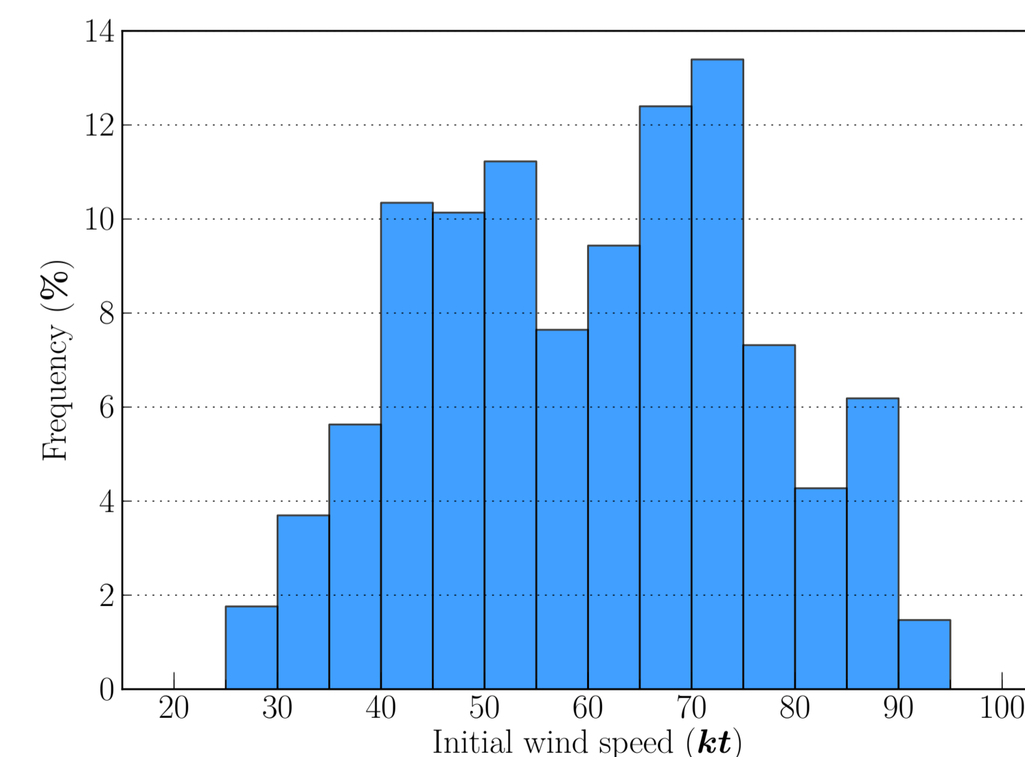
FIG. 2: The frequency of RI (number of cases per 5-kt bin over the total number of RI cases) as a function of the maximum wind speed of systems at t = 0 \text{ h} .
