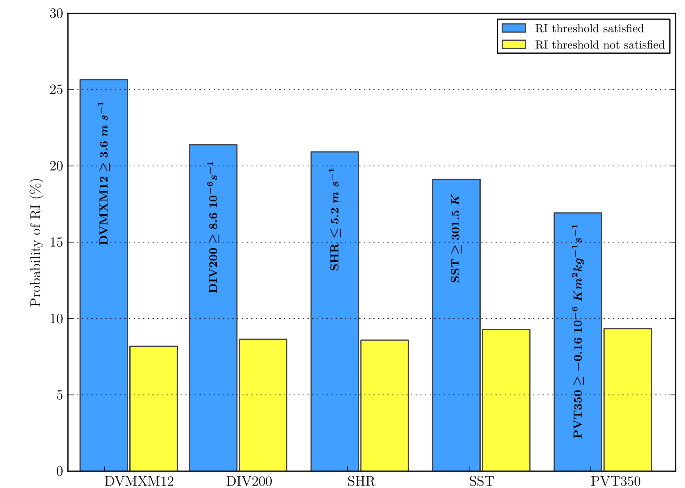
FIG. 3: The probability of RI when the specified predictors (X-axis) were satisfied (blue) or not (yellow) for the whole sample. RI thresholds for each variable (in blue columns) were determined as their means in the RI sample. To illustrate, RI occurred 25% (8%) of the time when DVMXM12 was above (below) the 3.6 \text{ m s}^{-1} threshold.
