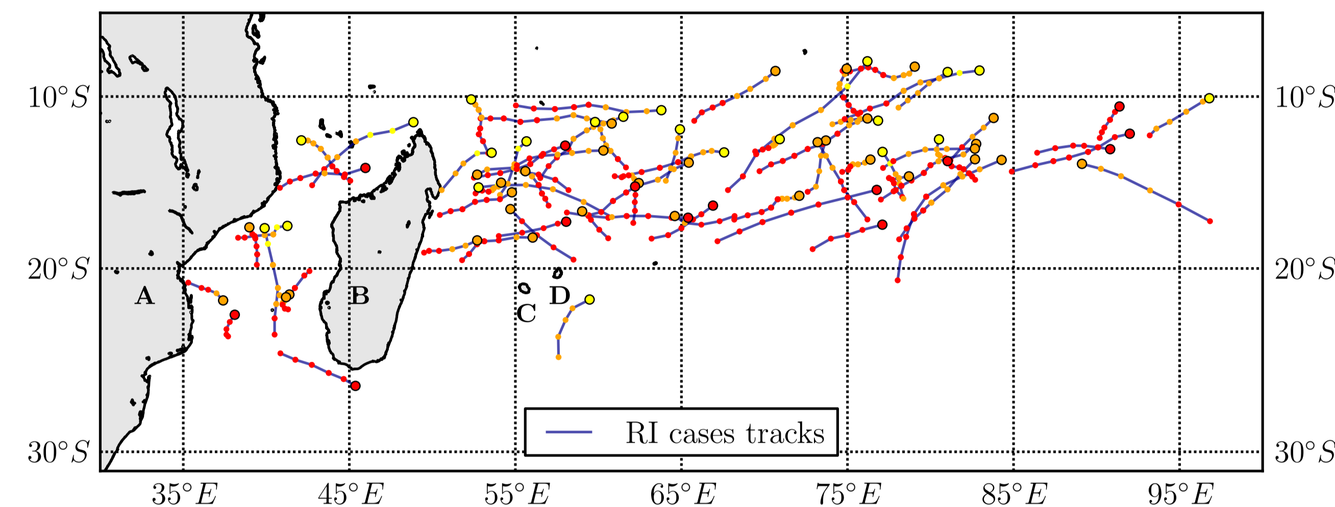
FIG. 1: 24-h tracks of all RI cases during the 15-year period; black circles indicate the start of each track; TDs are drawn in yellow, TSs in orange, TCs in red. Letters A, B, C, D indicate Africa, Madagascar, Reunion and Mauritius islands.
