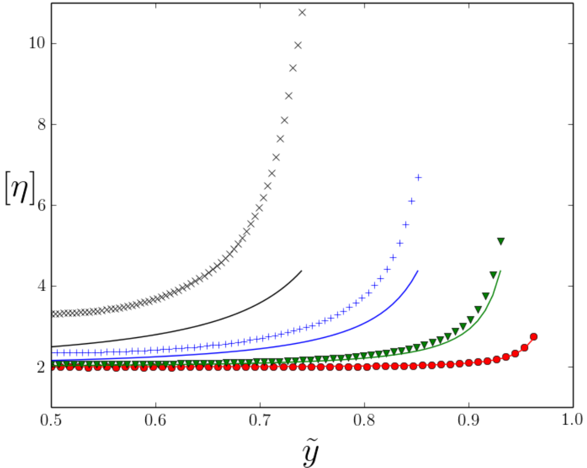
FIG. 2. Intrinsic viscosity depending on the dimensionless vertical position \tilde{y} for several confinements. For small confinements, when the particle is close to the middle of the channel ( \tilde{y} \approx 0.5 ) the asymptotic value [\eta] = 2 is recovered. For stronger confinements, even when the particle is centered ( \tilde{y} \approx 0.5 ), we get [\eta] > 2 . Red circles: C = 0.022 , green triangles: C = 0.0665 , blue +: C = 0.143 , black x: C = 0.25 . The analytical expansion [eq.(22)] (solid curves) fits quite well numerical results for small confinements ( C < 0.065 ).
