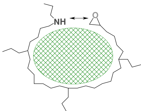
Scheme 9. Schematic representation of the sterical hindrance by Sn2 of the formation of the typical loops in a narrow network mesh, e.g. DGEBA-D230.
