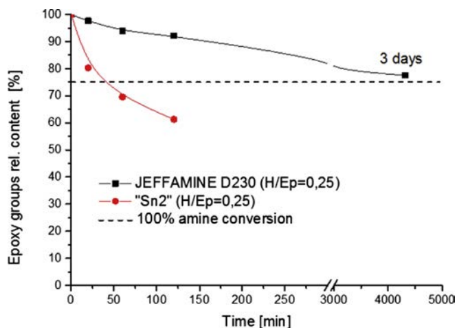
Fig. 1. Relative reactivity: kinetic curves of consumption of epoxy functions of phenyl glycidyl ether (which is chemically very similar to the epoxy component of the matrix, DGEBA), in reaction with the amino-functionalized nanofiller “Sn2” and with Jeffamine D230, a low-molecular-weight analogue of the amino component of the matrix. T = 120 °C, in sealed ampoule, r(\text{H}(-\text{N})/\text{Ep}) = 0.25 , c_0(\text{Ep}) = 1 M, c_0(\text{Am}) = 0.25 M, in toluene, epoxy groups are assumed to disappear by reaction with amine.
