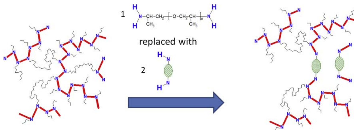
Scheme 5. Structure of the nanocomposite via replacement of a part of the branching and elastic amino-component of the matrix by the linearly bonded amino-functional stannoxane nanofiller Sn2.
