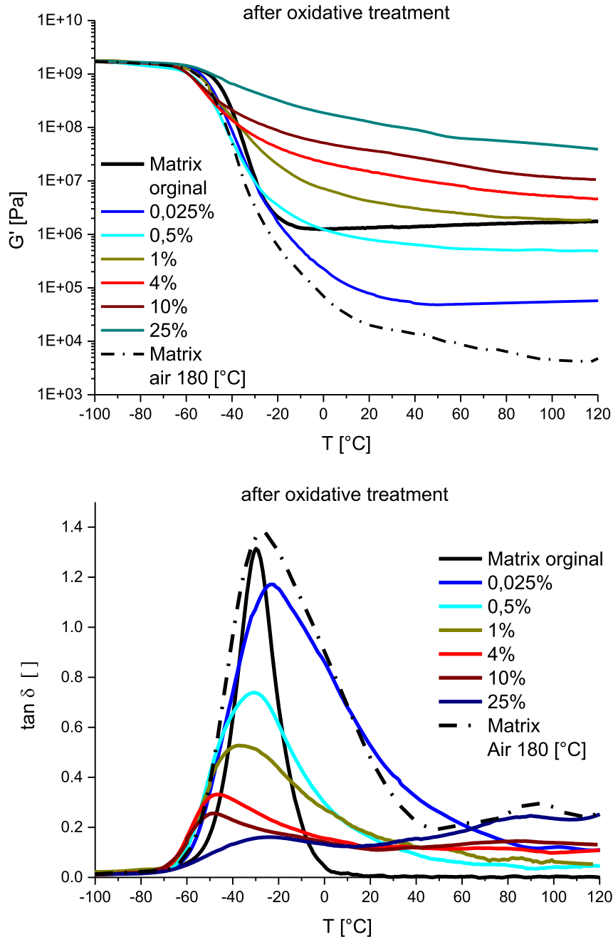
Fig. 11. Effect of nanofiller content on the thermo-mechanical properties of the epoxy-Sn2 nanocomposites which underwent oxidation treatment: Shear storage modulus G' (top) and loss factor \tan(\delta) (bottom) as function of temperature: nanofiller content is in the range of 0.025–25 mol% amino protons.
