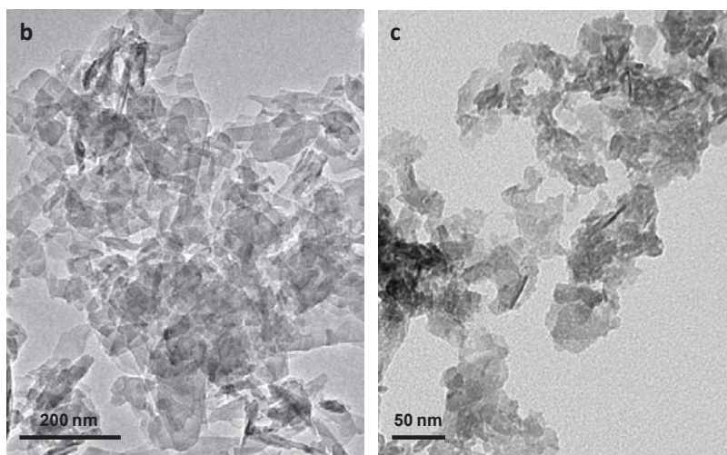
Figure S2/ The samples CHA and CHA-SBF are biomimetic apatites. The CHA and CHA-SBF are apatite samples possessing a low degree of crystallinity similar to the bone mineral as shown by XRD (no contaminant phase is detected) (a). Standard TEM observations of CHA and CHA-SBF powders. They are formed of nanometric platelets as bone mineral. The size is polydispersed for CHA with an average of 200 \times 100 \times 5 \text{ nm}^3 (b) whereas CHA-SBF platelets are smaller and more homogeneous in size with an average of 50 \times 50 \times 2-4 \text{ nm}^3 (c).
