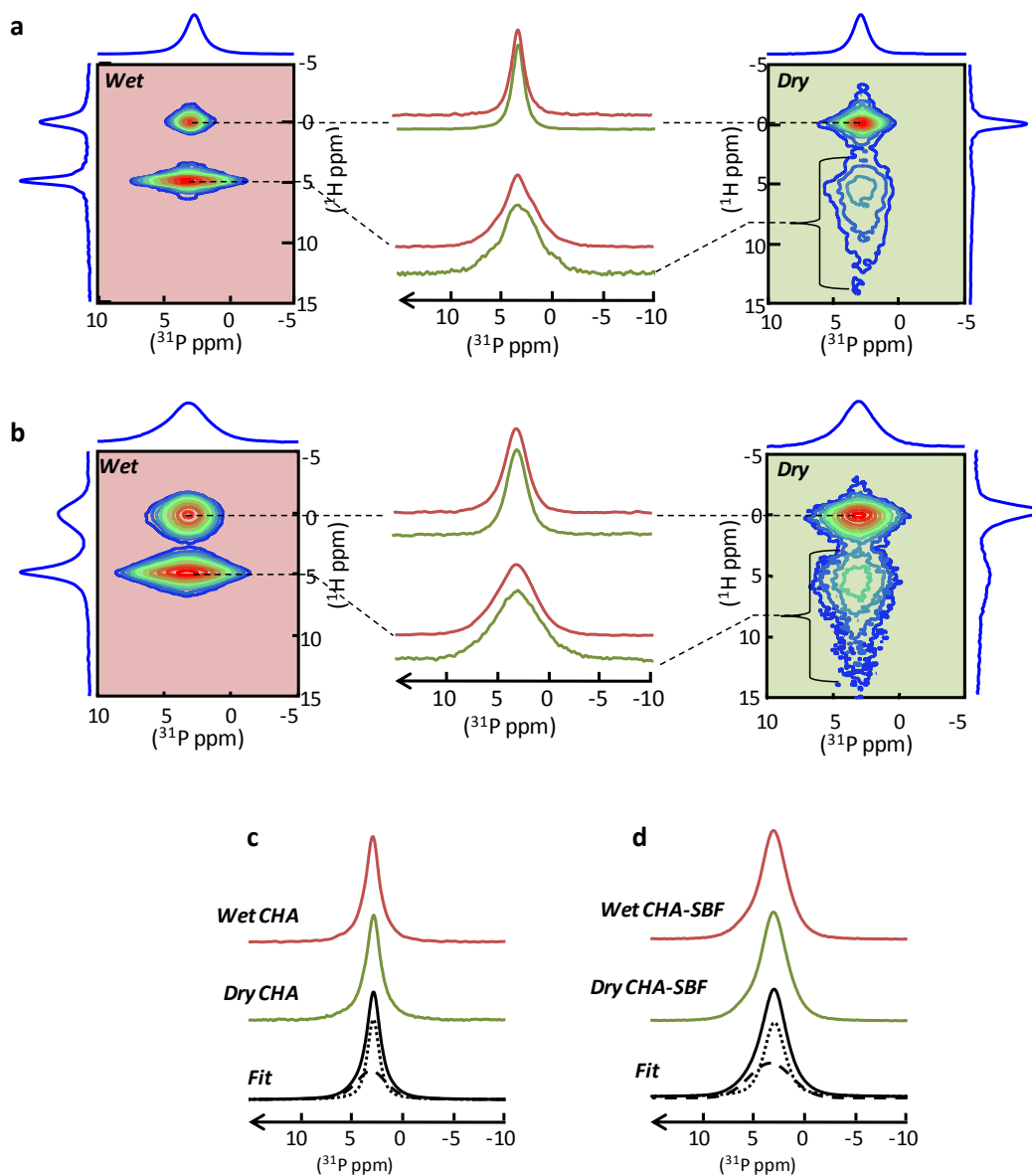
Figure S3/ a-b , 2D ^1\text{H} - ^{31}\text{P} HetCor experiments (contact time CT = 1 ms) of CHA (a) and CHA-SBF (b) particles in dry (green) and H 2 O soaked (red) conditions. Two correlation peaks are detected and correspond to (i) ^{31}\text{P} from the apatitic core (signing with the hydroxyls at \delta(^1\text{H}) = 0 ppm) and (ii) ^{31}\text{P} at the hydrophilic surface which is signing with the sharp resonance of adsorbed water molecules ( \delta(^1\text{H}) = 4.85 ppm) in the hydrated state and with the broader resonance of POH and residual water molecules (5-15 ppm) in the dry state. c-d , The ^{31}\text{P} MAS spectra recorded on hydrated (red) and dry (green) CHA (c) and CHA-SBF (d) are
