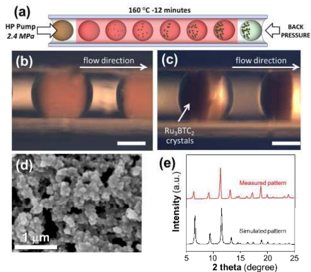
Figure 4. (a) Schematic representation of hydrothermal microchemical process. Optical images of single microdroplets containing (b) completely dissolved precursor solution and (c) segregated Ru_3BTC_2 crystals in the droplet after 12 min of synthesis at 160\text{ }^\circ\text{C} and 2.4\text{ MPa} (scale bar: 100\text{ }\mu\text{m} ). (d) SEM micrograph and (e) XRD pattern of the obtained crystals, which is compared with the simulated pattern from the single-crystal XRD of Ru_3BTC_2 .
