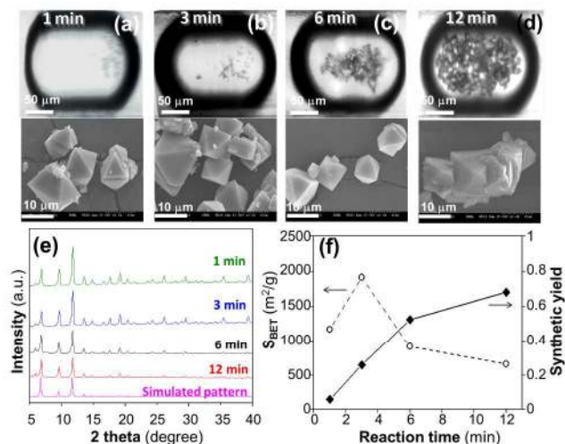
Figure 2. Optical and SEM micrographs of HKUST-1 crystals obtained via the microfluidic approach after (a) 1, (b) 3, (c) 6, and (d) 12 min of synthesis, [Cu] = 0.12 M. (e) The corresponding XRD patterns, which are compared with the simulated pattern from single-crystal XRD data of HKUST-1, and (f) the synthetic yield (bold line) and BET surface area, S BET (dotted line) as a function of reaction time.
