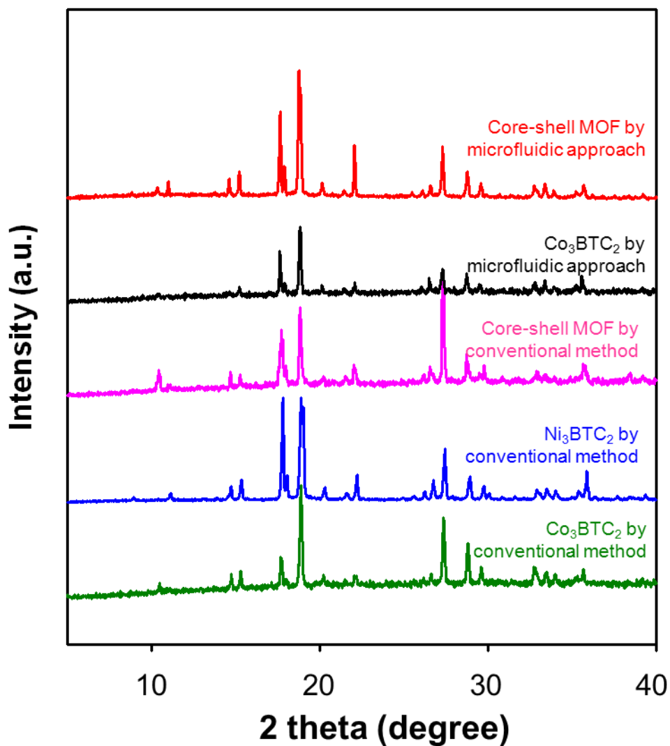
Figure S7. Powder X-ray diffraction patterns of \text{Co}_3\text{BTC}_2 , \text{Ni}_3\text{BTC}_2 and \text{Co}_3\text{BTC}_2@ \text{Ni}_3\text{BTC}_2 obtained from both conventional and microfluidic approach.
