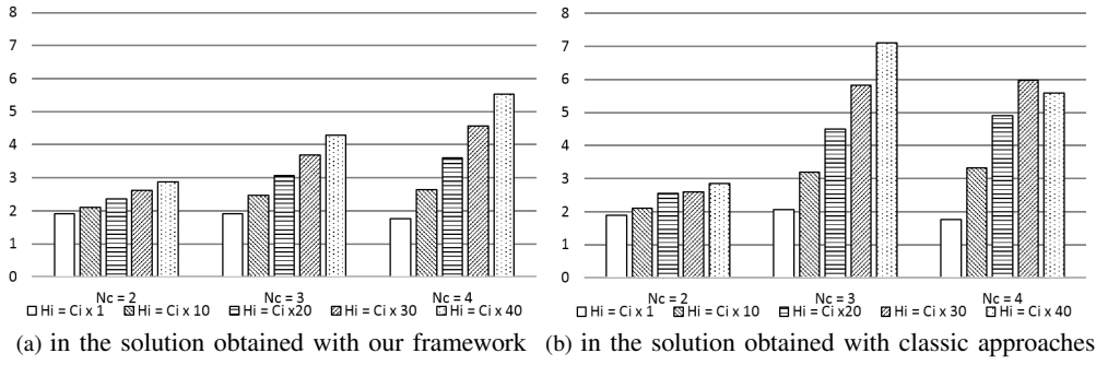
Fig. 4: average workload per core (%)
