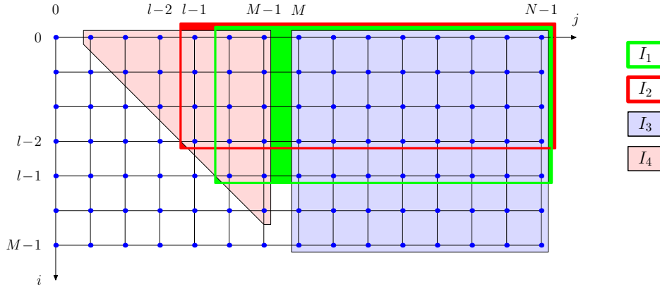
Figure 5: Rotations indexes for m < d < m(M-1) , d \neq lm .
