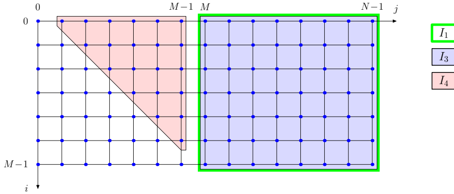
Figure 2: Rotations indexes for d = mM .
