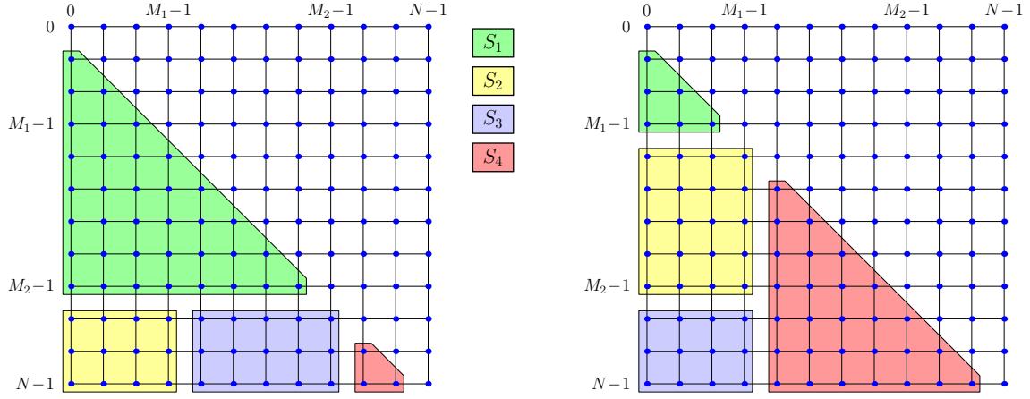
Figure 1: The sets S_i, 1 \leq i \leq 4 at left for relation (3.22), at right for (3.23).
