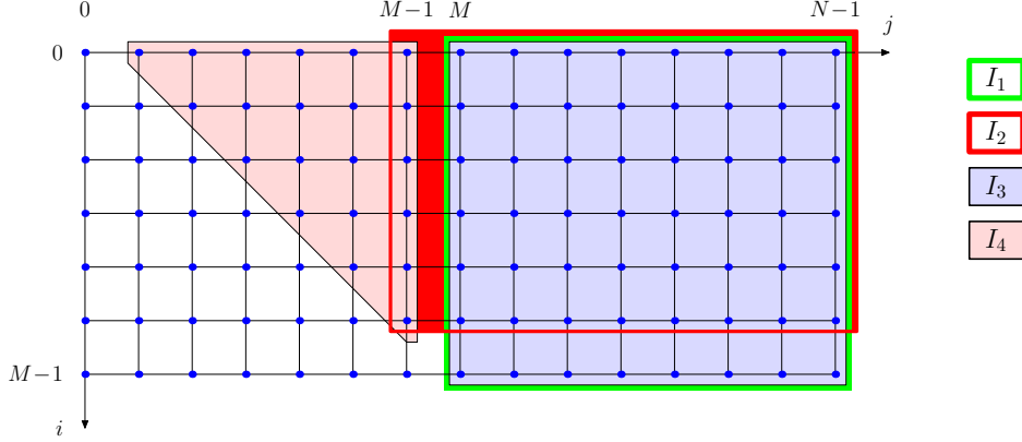
Figure 3: Rotations indexes for m(M-1) < d < mM .
