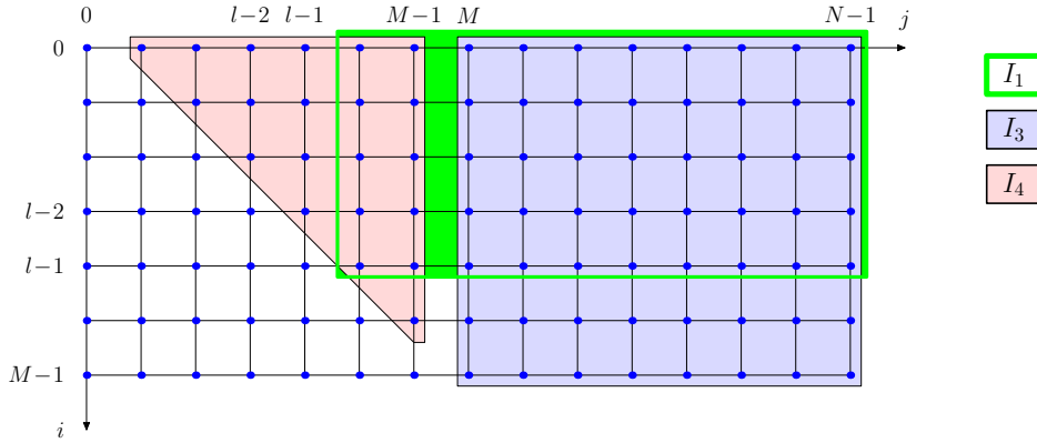
Figure 4: Rotations indexes for d = lm , 1 \leq l < M .
