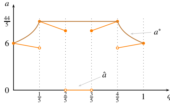
Figure 6: Functions a^* and \hat{a} for example 2
