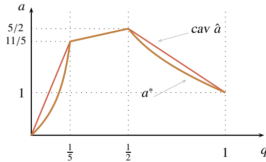
Figure 5: Functions a^* and \text{cav } \hat{a} for Example 1
