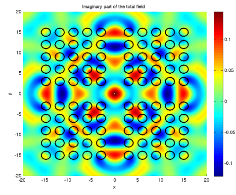
(e) Imaginary part of the total field
