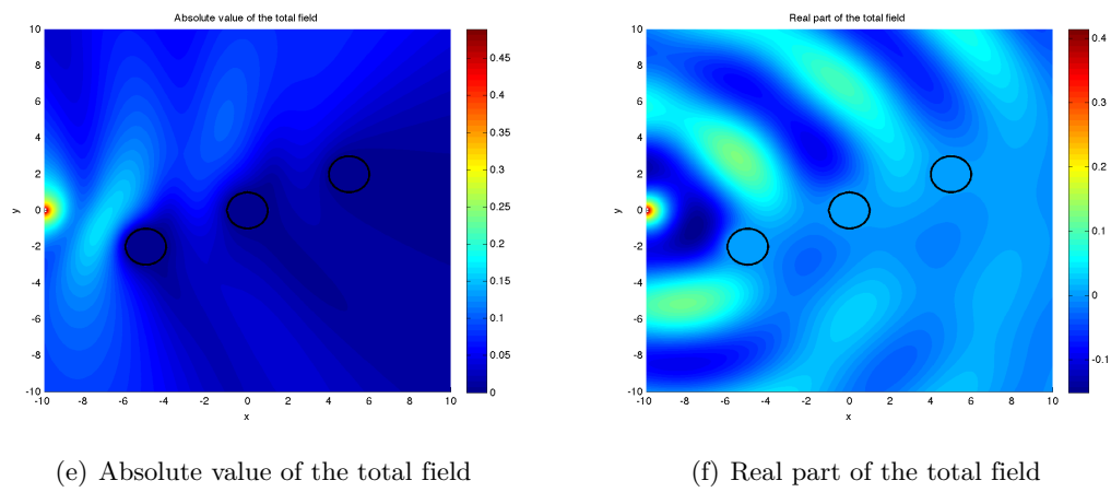
Figure 4.2: Different results for a Dirichlet problem for a wave emitted by a point source solved using \mu -diff. The first two pictures show respectively the obstacles and the radar cross section, while the third one shows the GMRES history of convergence. The absolute value of the scattered field is presented on subfigure (d), and the total field on figures (e) (absolute value) and (f) (real part).
