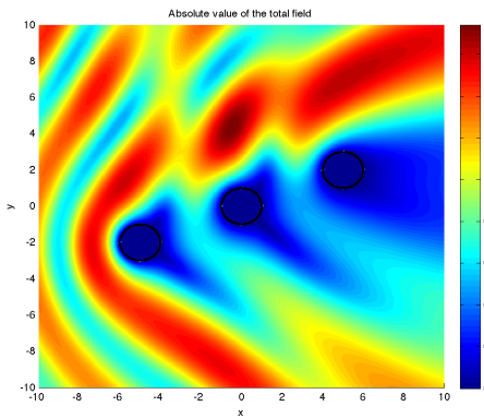
(e) Absolute value of the total field
