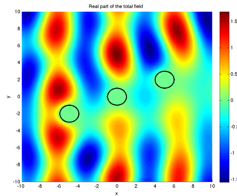
(f) Real part of the total field
