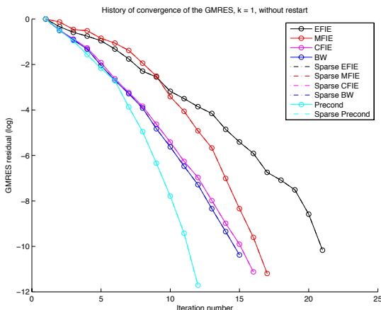
(c) History of convergence of the GMRES
