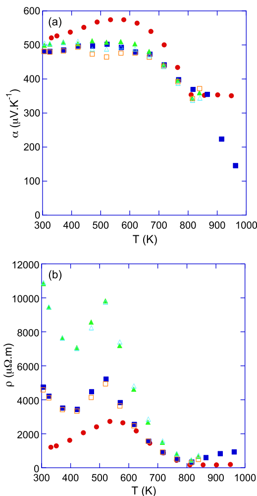
FIG. 3. Temperature dependence of the electrical properties of SnSe measured in both directions: (a) thermopower \alpha and (b) electrical resistivity \rho . Both properties were measured parallel (triangle symbols) and perpendicular (square symbols) to the pressing direction in two different samples (sample 1 filled symbols and sample 2 open symbols). The mean value of the data collected on single crystals has been added for comparison (filled circle symbols).
