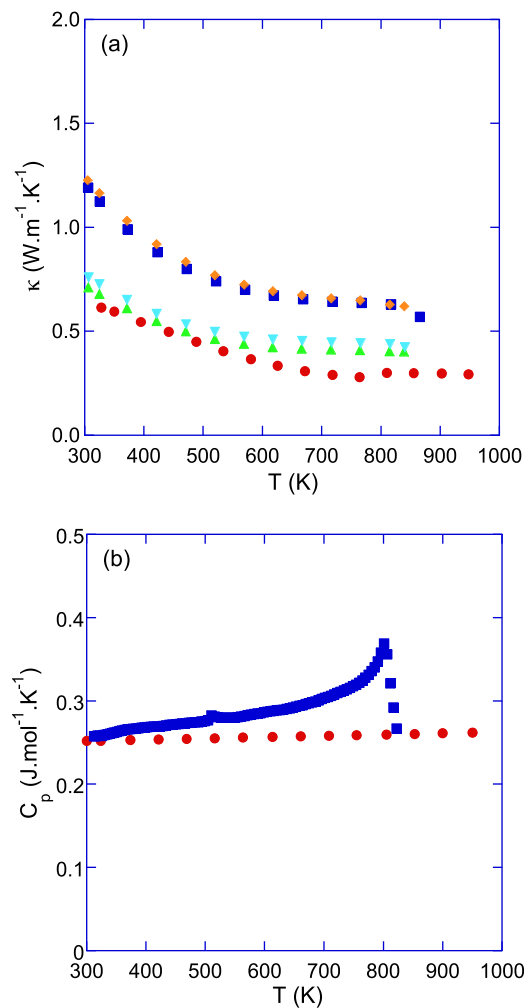
FIG. 4. (a) Temperature dependence of the total thermal conductivity \kappa of polycrystalline bulk samples of SnSe measured parallel and perpendicular to the pressing direction. The mean value of the data obtained on single crystals by Zhao et al. 11 has been added for comparison. (b) Specific heat data as a function of temperature in polycrystalline (square symbol) and single-crystalline (circle symbol) samples. The anomaly around 504 K corresponds to the melting temperature of elemental Sn in agreement with SEM analyses. The second anomaly at 800 K might be related to the structural transition. Note that we have extrapolated the temperature dependence of the specific heat linearly from 300 up to 820 K to calculate \kappa .
