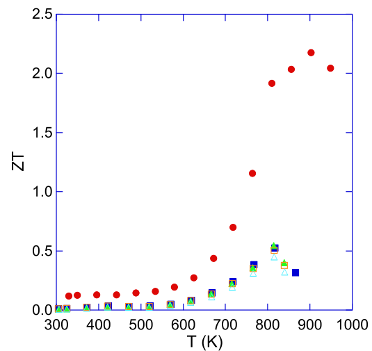
FIG. 5. Temperature dependence of the dimensionless figure of merit ZT of polycrystalline bulk samples of SnSe measured parallel and perpendicular to the pressing direction compared with the values obtained in single crystals.
