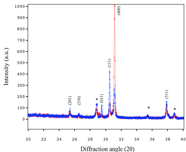
FIG. 1. Magnification of XRPD patterns around the main Bragg peaks measured on bulk samples parallel (blue color) and perpendicular (red color) to the pressing direction. The (hkl) values are indicated for each reflection. The asterisk corresponds to extrinsic reflections coming from the sample holder.
