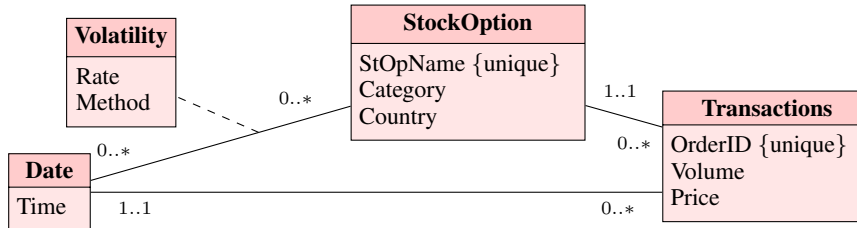
Figure 1: Data model for stock exchange information
