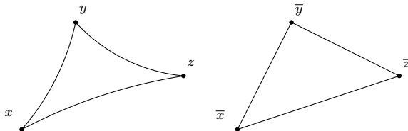
Figure 1: A geodesic triangle in a CAT(0) space is thinner than a triangle in the Euclidean plane with same side lengths.
