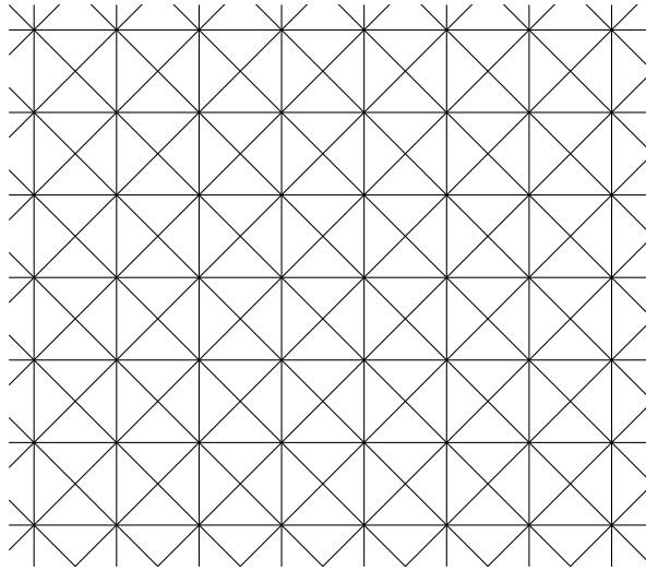
Figure 3: Reflections hyperplanes for the discrete affine Weyl group B_2 \times \mathbb{Z}^2 .
