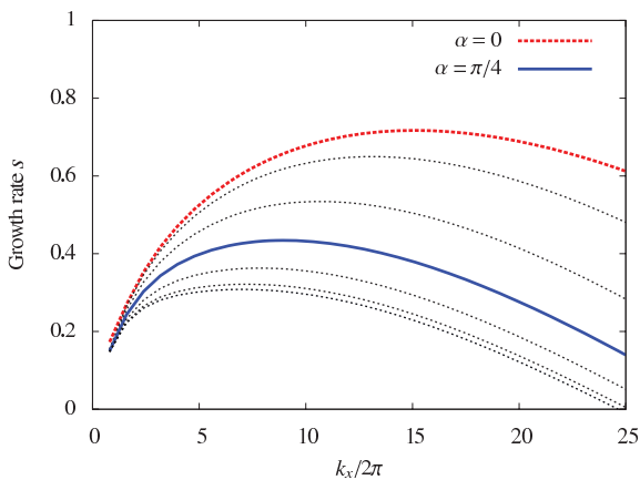
Figure 3. Growth rate s of the instability versus horizontal wavenumber k_x for the initial configuration presented in Fig. 2. The results are presented for different angles \alpha from 0 (unidirectional field) to \pi/2 (the field lines are perpendicular). We stress the case \alpha = \pi/4 as it is the largest value considered numerically in the text.
