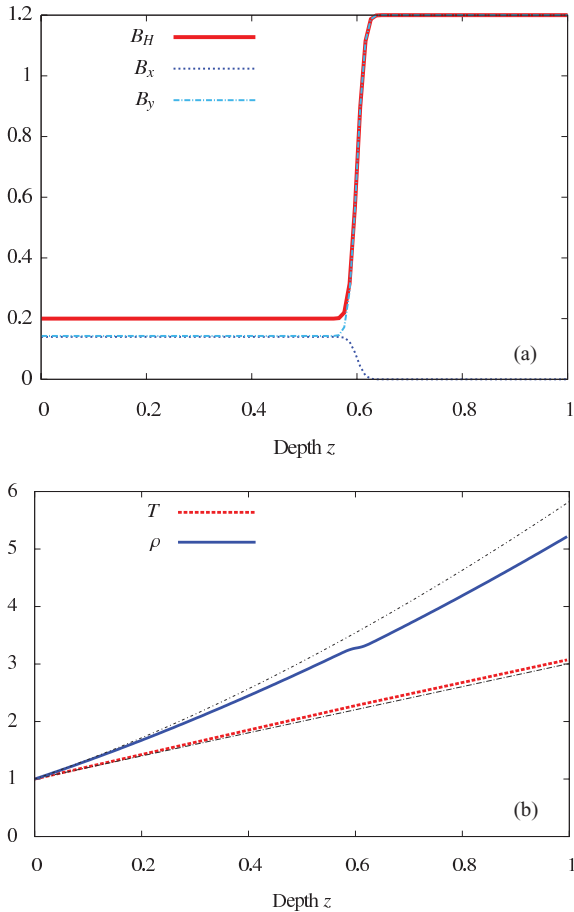
Figure 2. Initial condition for the horizontal components of the magnetic field, the temperature, T , and the density, \rho . In the top image, the dashed lines correspond to the vertical profile of B_x and B_y for the particular case \alpha = \pi/4 . In the bottom image, the dashed lines represent the basic state of temperature and density in the absence of a magnetic field. The parameter F has been increased from F = 0.1 (the value used in this paper) to F = 1 in order to enhance the modifications of the basic field-free polytropic state.
