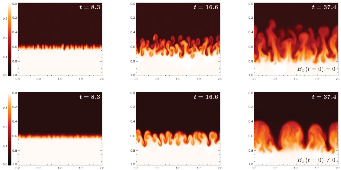
Figure 4. Evolution of the instability in the (x,z) plane perpendicular to the initial field lines in the layer. In the upper row, the magnetic field lines are unidirectional and directed perpendicularly to the plane of visualization. In the lower row, the field lines for z < 0.6 are orientated at 45^\circ with respect to the field lines inside the layer. Bright colours correspond to the strong B_y field, whereas dark tones correspond to the weaker field. Time is increasing from left to right: t = 8.3, 16.6 and 37.4 .
