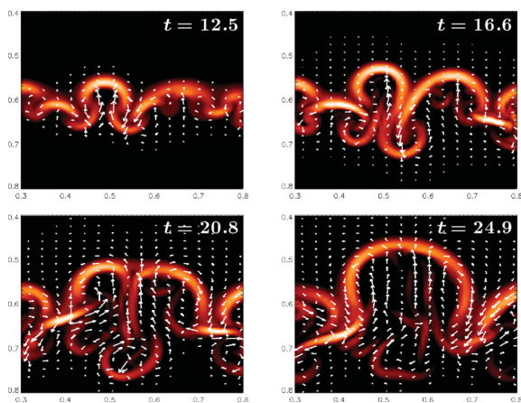
Figure 5. Details of the merging mechanism. The contours show the current density j^2 in a small part of the (x, z) plane for different times. Dark tones correspond to weak current, whereas light colours correspond to strong current. The same colour scale is used for the different times. The velocity field in the plane (x, z) is also shown as arrows whose length depends on the velocity amplitude.
