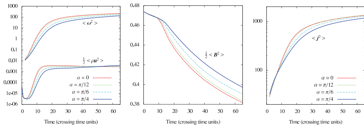
Figure 7. Evolution of the total kinetic energy, enstrophy, magnetic energy and current density versus time for four different angles from \alpha = 0 to \pi/4 .
