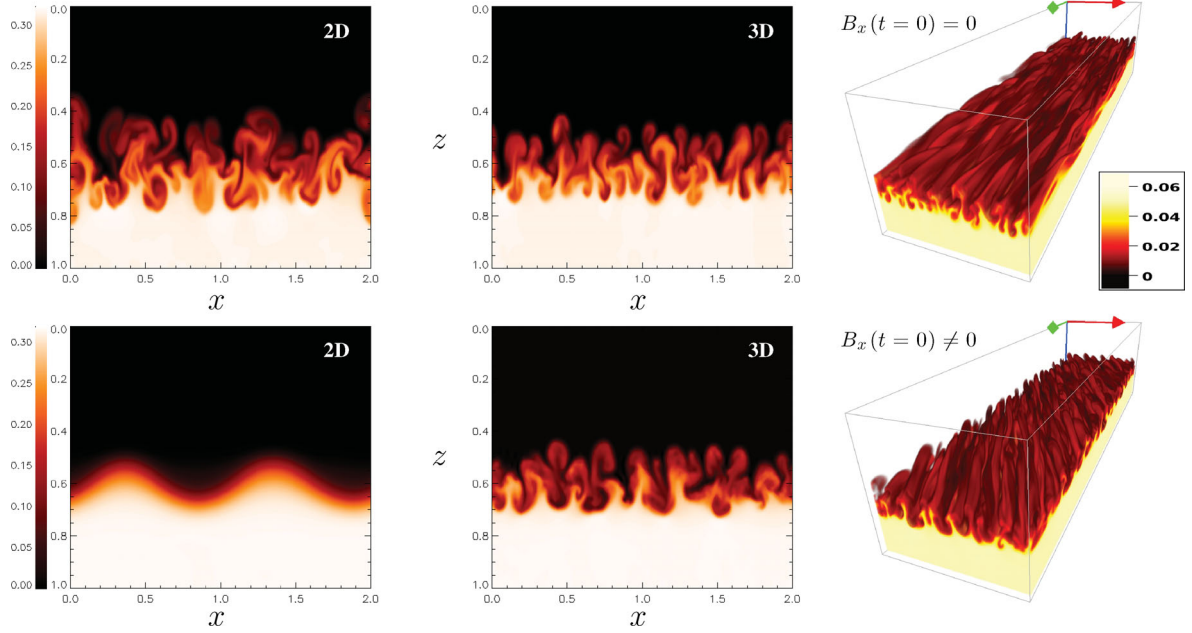
Figure 1. Comparison between 2D and 3D simulations. Top line: the initial field is unidirectional, directed perpendicularly to the plane. Bottom line: the initial magnetic layer is sheared. In the left column, we show contours of B_y from the 2D simulations, whereas the middle column corresponds to one particular (x, z) plane inside the 3D domain. In the right column, we show a volume rendering of the magnetic energy from the 3D simulations at the same time. All visualizations are performed at the same time t \approx 20 , except for the bottom-left figure, which corresponds to t \approx 50 (due to the fact that the growth rate of the instability is strongly reduced in this particular case; see, for example, Cattaneo et al. 1990a).
