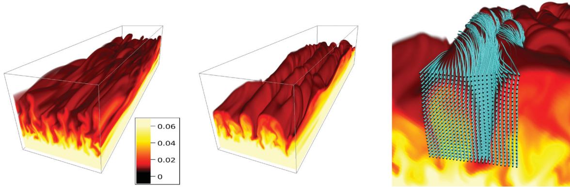
Figure 6. Volume rendering of the magnetic energy. The case \alpha = 0 is presented on the left, whereas the case \alpha = \pi/4 is shown in the middle. The visualizations are realized at the same time t = 24 . The figure on the right presents a subvolume of the case \alpha = \pi/4 where magnetic field lines have been added in order to enhance the twisted nature of the field.
