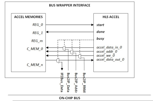
Fig. 2. Generic bus wrapper interface to let a HLS generated accelerator connect an on-chip bus.
