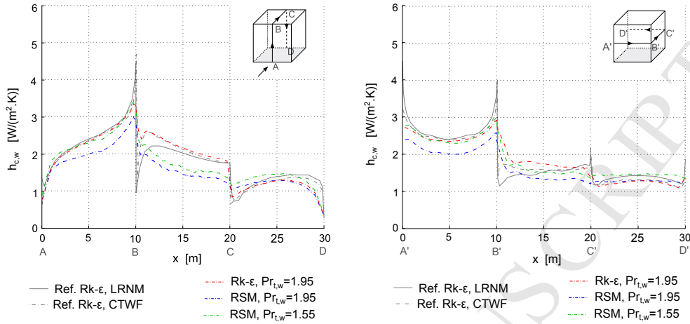
Figure 5: Comparison of the h profiles obtained using customized Pr_{t,w} values with reference (Ref.) R- k - \varepsilon LRNM data [41].
