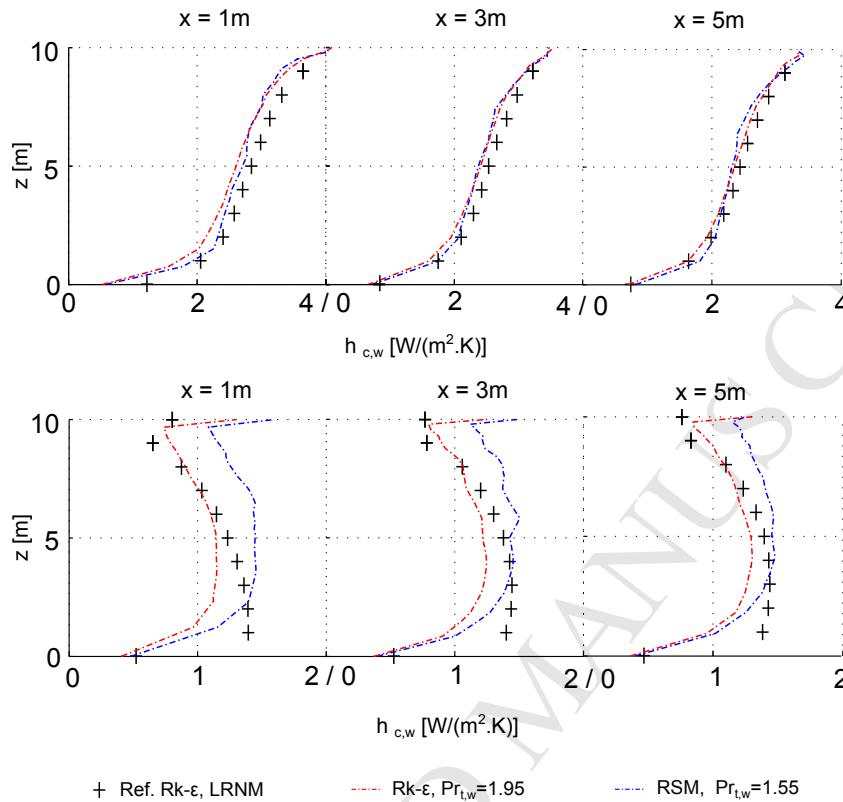
Figure 6: Comparison between the simulated h profiles using the R- k - \epsilon model with Pr_{t,w} = 1.95 or the RSM - CTWF with Pr_{t,w} = 1.55 with reference LRNM [41] on the front (top) and rear (bottom) faces of the cubical building and for U_{10} = 0.5\text{ m} \cdot \text{s}^{-1} .
