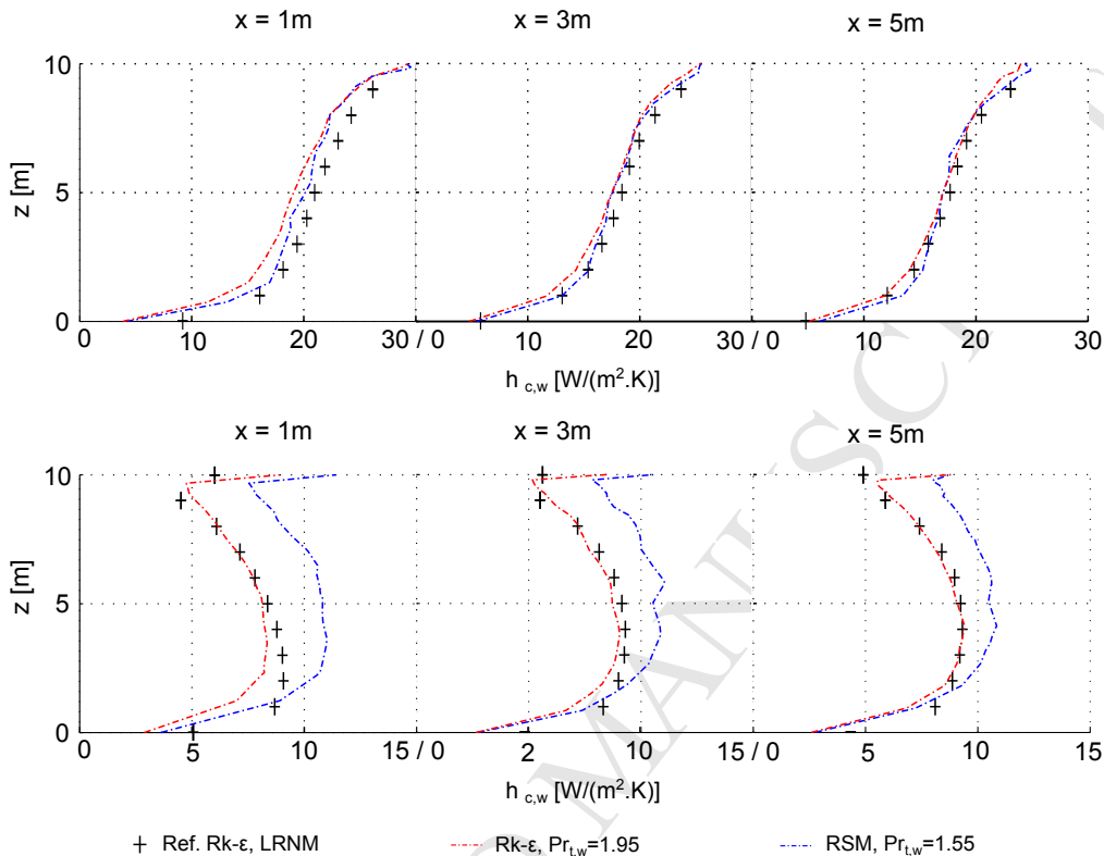
Figure 7: Comparison between the simulated h profiles using the R- k - \varepsilon or RSM - CTWF with reference LRNM data [41] on the front (top) and rear (bottom) faces of the cubical building and for U_{10} = 5 \text{ m} \cdot \text{s}^{-1} .
